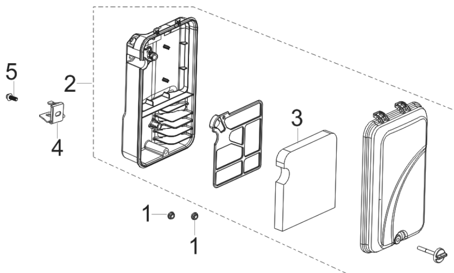
FIG.12 CLEANER, AIR (F01)
