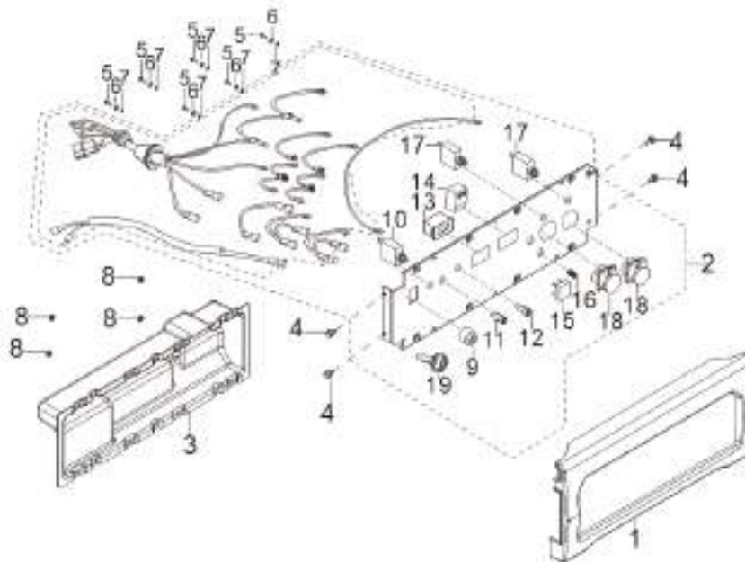
FIG.17 PANEL SUBASSEMBLY, CONTROL (F05)
