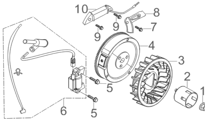
FIG.10 FLYWHEEL / IMPELLER / STARTER PULLEY / IGNITION COIL (E10)
