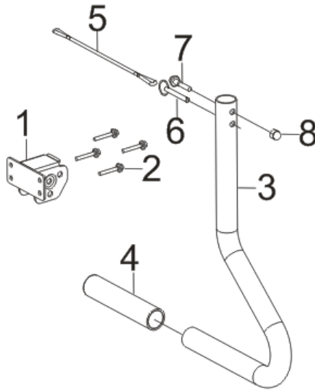
FIG20: HANDLE ASSY (F08)
