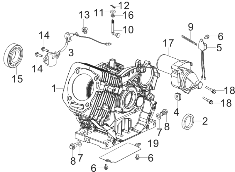
FIG.1 CRANKCASE. / GEAR ASSY, GOVERNOR. (E01)
