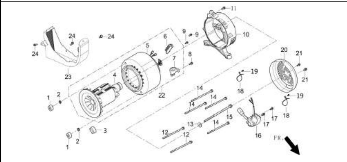
FIG.18 ROTOR/STATOR (F06)
