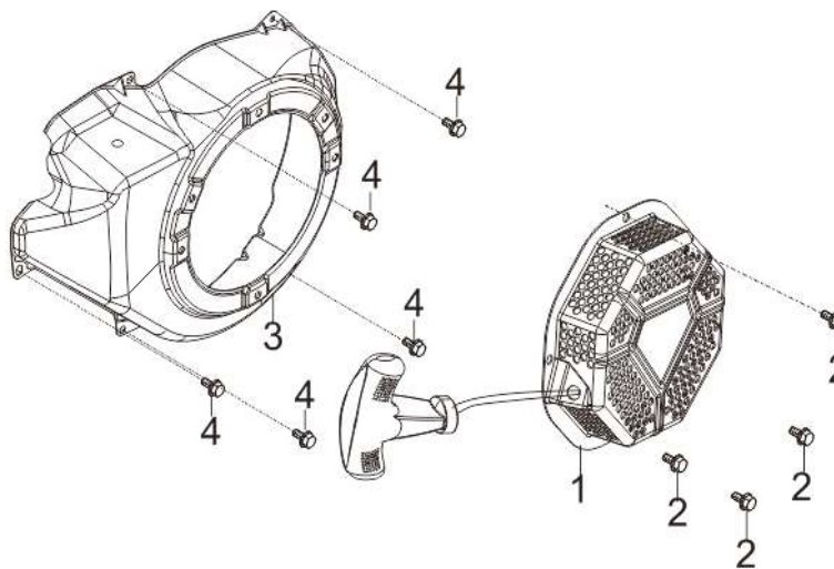
FIG.7 STARTER,RECOIL (E07)
