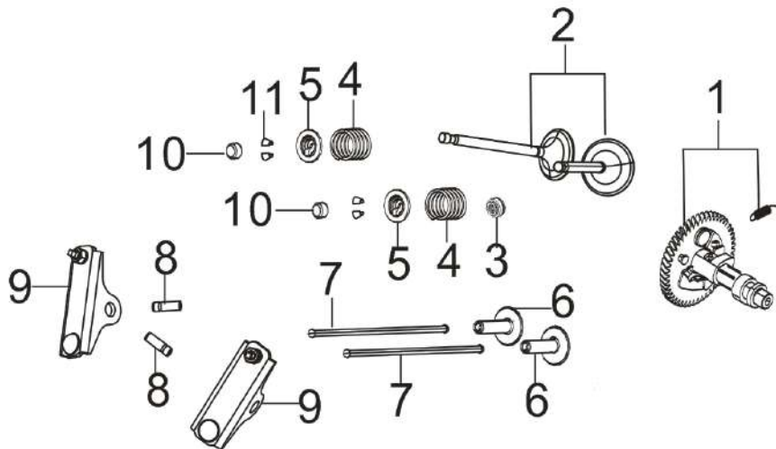
FIG.6 TRAIN,VALVE / CAMSHAFT SUBASSEMBLY (E06)
