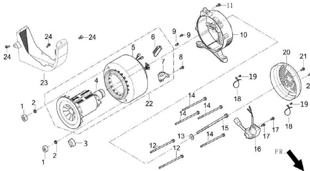
FIG.16 ROTOR/STATOR (F06)
