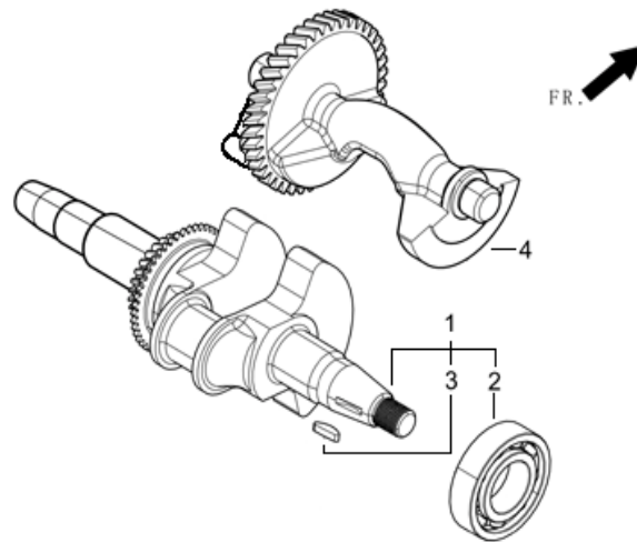
FIG.4 ROD,CRANKSHAFT CONNETING (E04)
