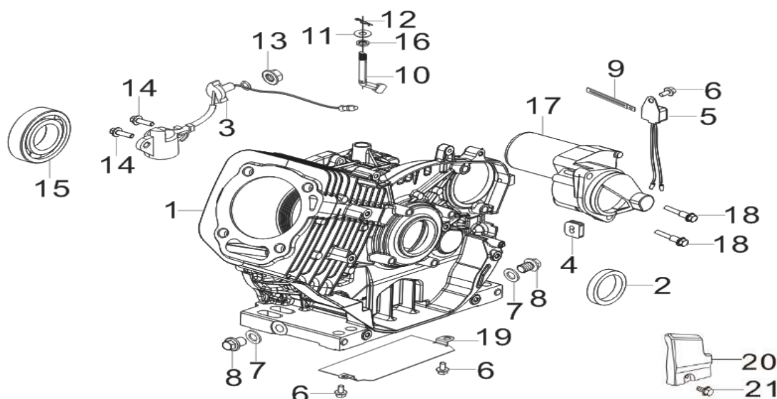
FIG.1 CRANKCASE. / GEAR ASSY, GOVERNOR. (E01)
