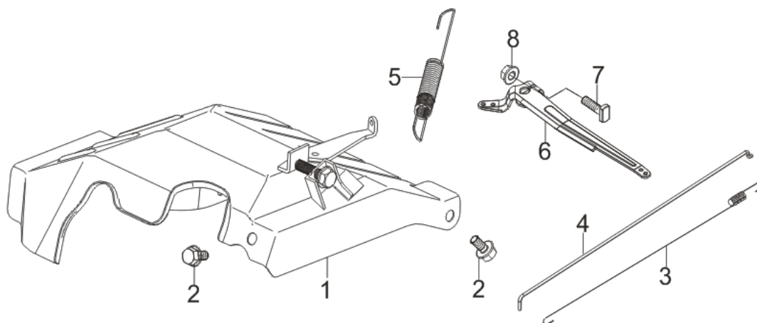
FIG.10 CONTROL ASSY, THROTTLE (E11)
