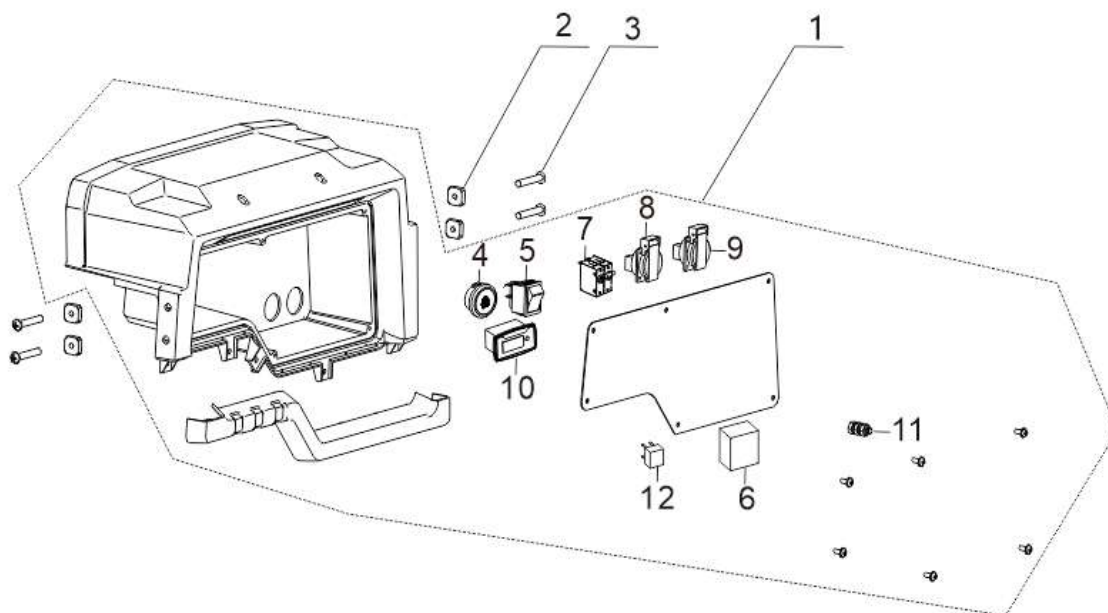
FIG.15 PANEL SUBASSEMBLY, CONTROL (F05)
