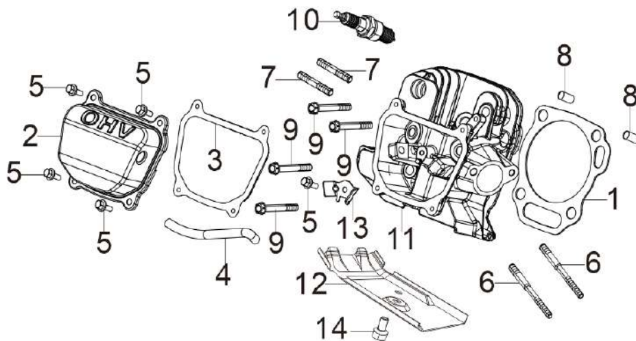
FIG.3 HEAD SUBASSEMBLY, CYLINDER / PLUG,SPARK (E03)
