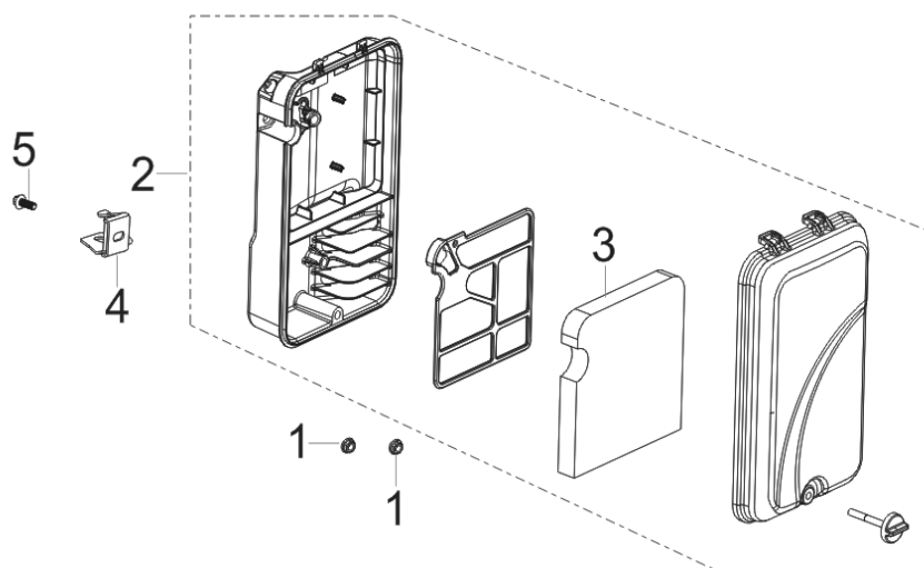
FIG.11 CLEANER, AIR (F01)
