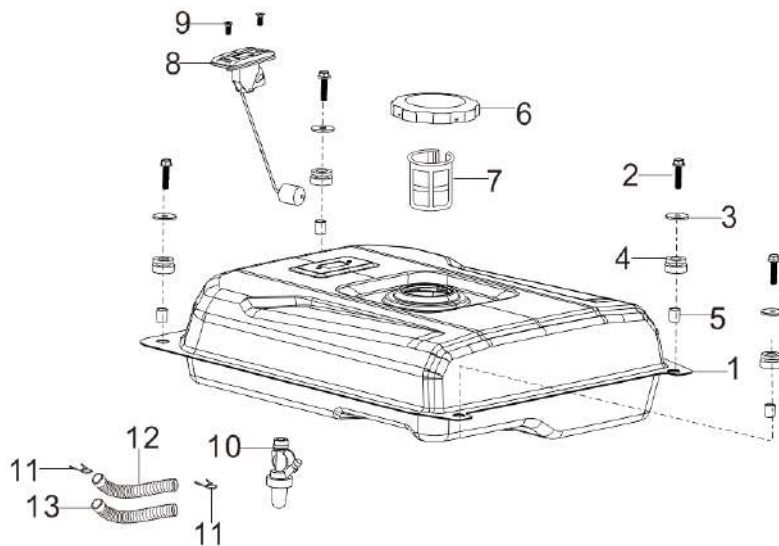
FIG.13 TANK ASSY, FUEL (F03)
