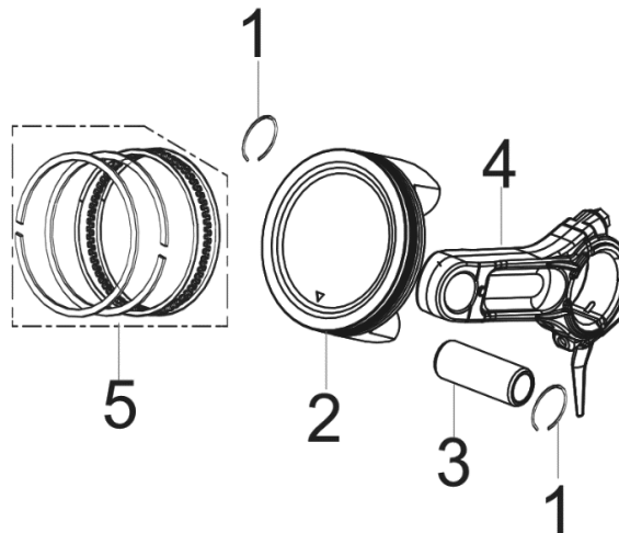
FIG.5 RING SET,OIL / ROD,CRANKSHAFT CONNETING (E05)
