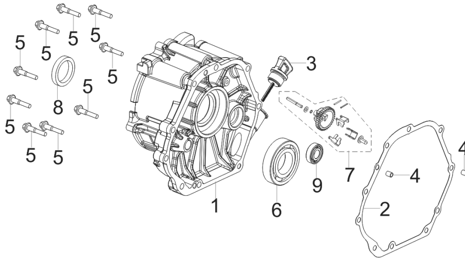
FIG.2 COVER SUBASSEMBLY, CRANKCASE (E02)
