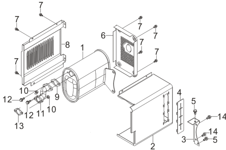
FIG.14 MUFFLER ASSY. (F02)
