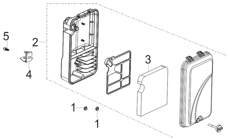
FIG.12 CLEANER, AIR (F01)
