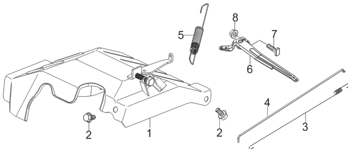
FIG.11 CONTROL ASSY, THROTTLE (E11)
