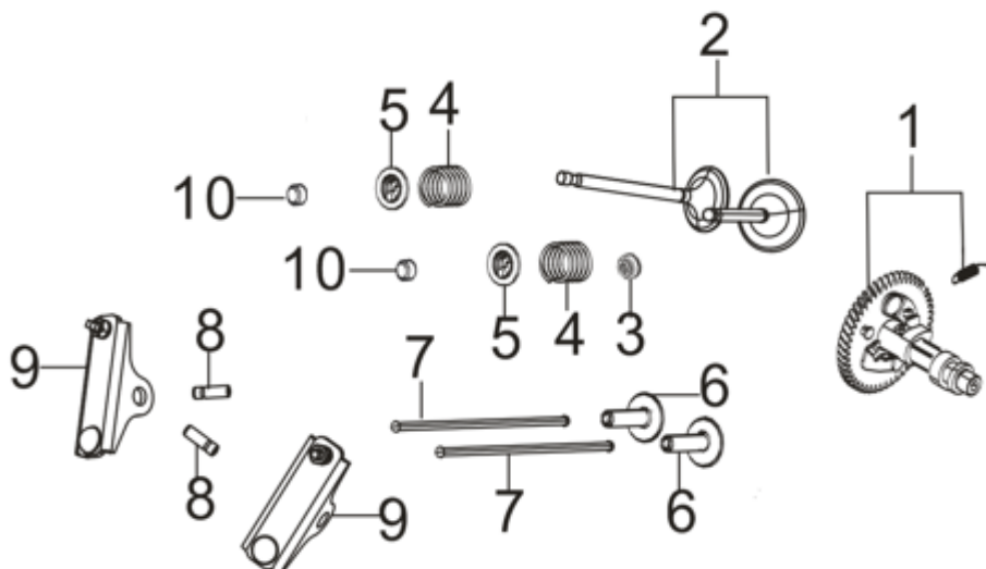
FIG.6 TRAIN,VALVE / CAMSHAFT SUBASSEMBLY (E06)
