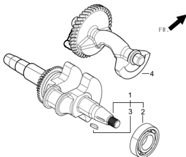
FIG.4 ROD,CRANKSHAFT CONNETING (E04)
