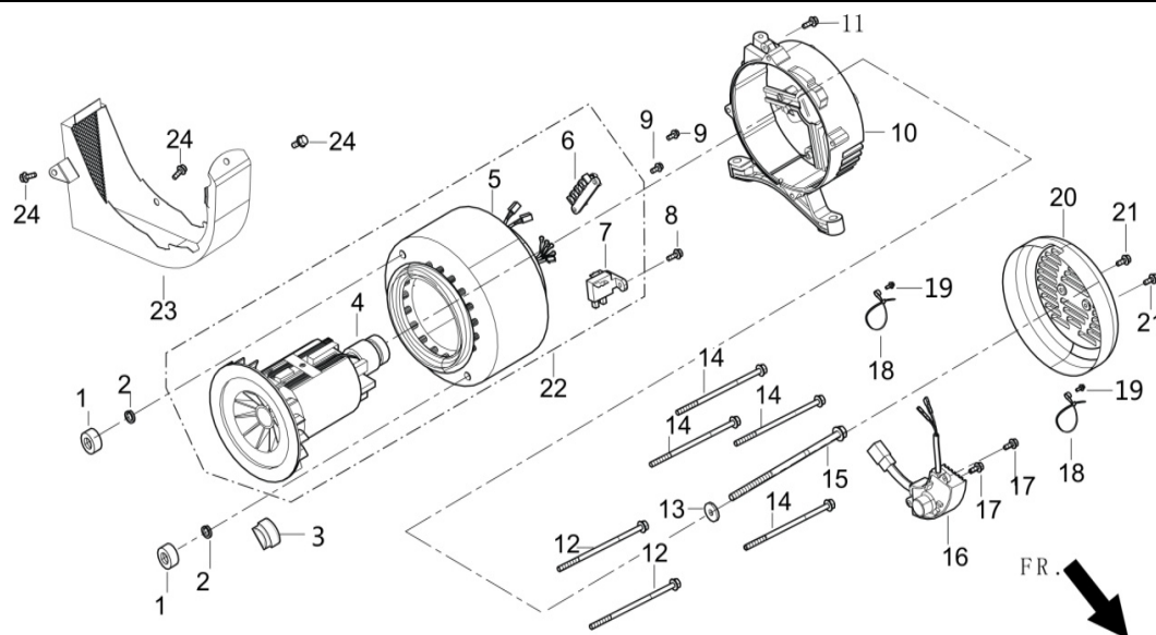
FIG.18 ROTOR/STATOR (F06)
