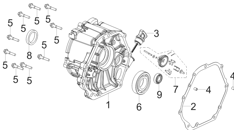
FIG.2 COVER SUBASSEMBLY, CRANKCASE (E02)
