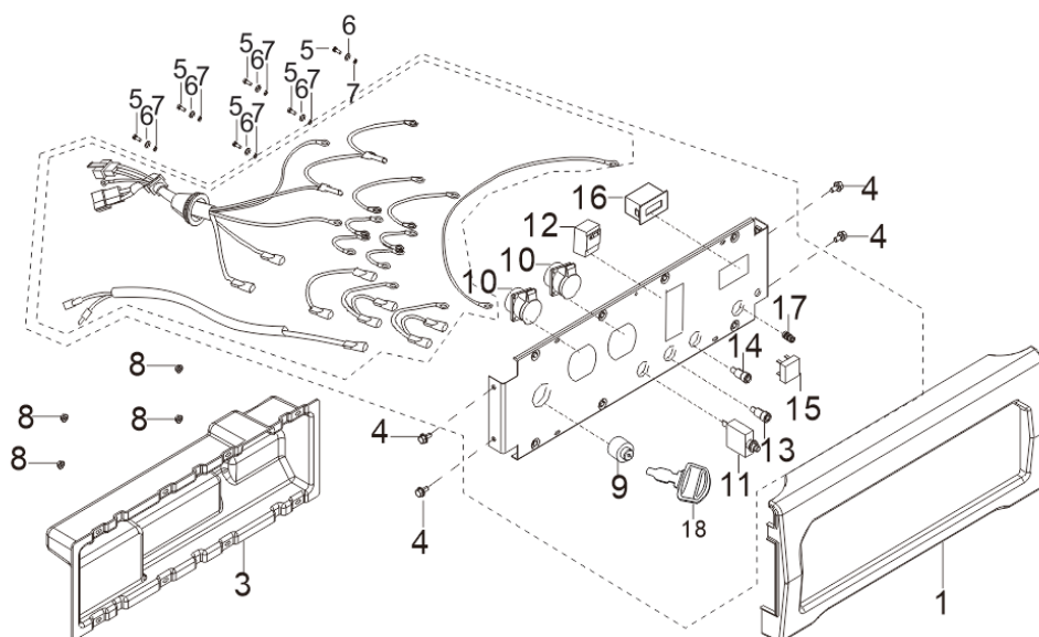
FIG.17 PANEL SUBASSEMBLY, CONTROL (F05)
