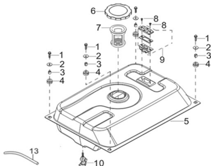
FIG.15 TANK ASSY, FUEL (F03)
