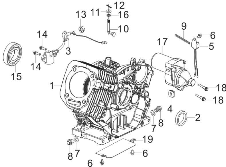
FIG.1 CRANKCASE. / GEAR ASSY, GOVERNOR. (E01)
