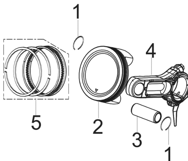
FIG.5 RING SET,OIL / ROD,CRANKSHAFT CONNETING (E05)
