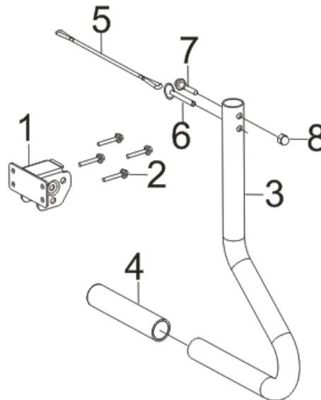
FIG.20: HANDLE ASSY (F08)
