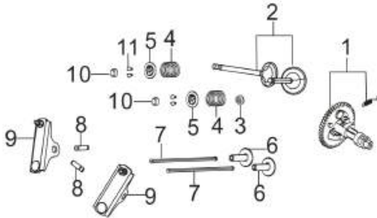
FIG.6 TRAIN,VALVE / CAMSHAFT SUBASSEMBLY (E06)
