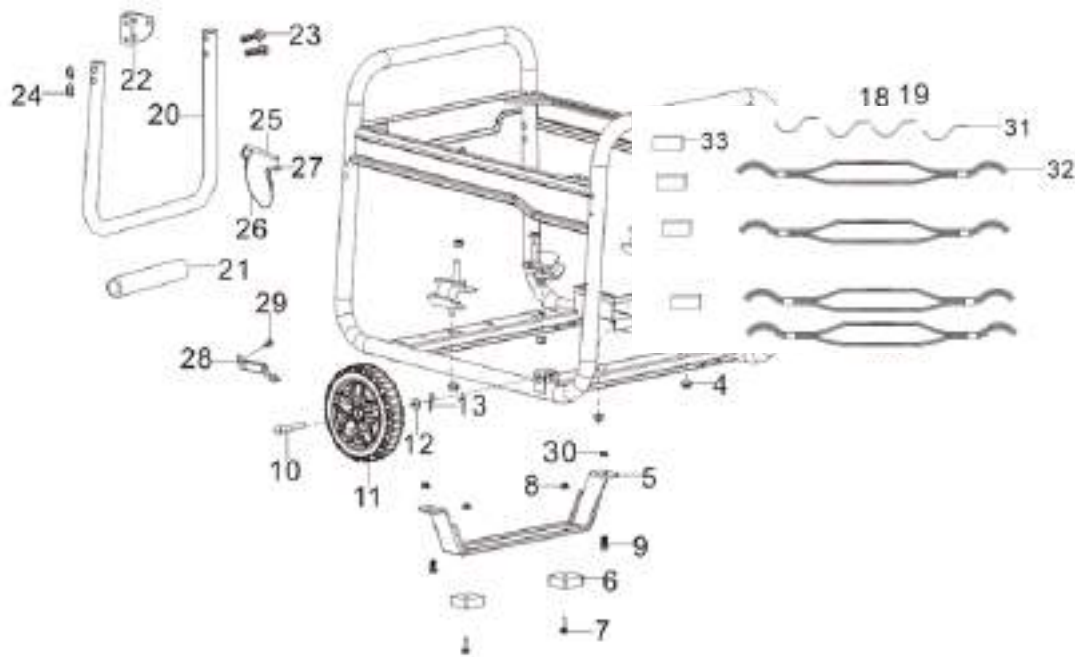
FIG.14 FRAME, ENGINE ( F04 )
