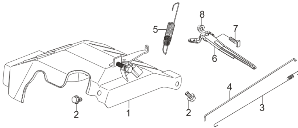
FIG.10 CONTROL ASSY, THROTTLE (E11)
