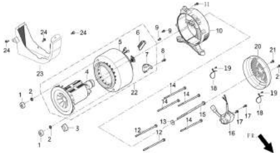
FIG.16 ROTOR/STATOR (F06)
