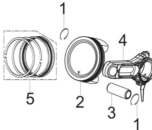
FIG.5 RING SET,OIL / ROD,CRANKSHAFT CONNETING (E05)
