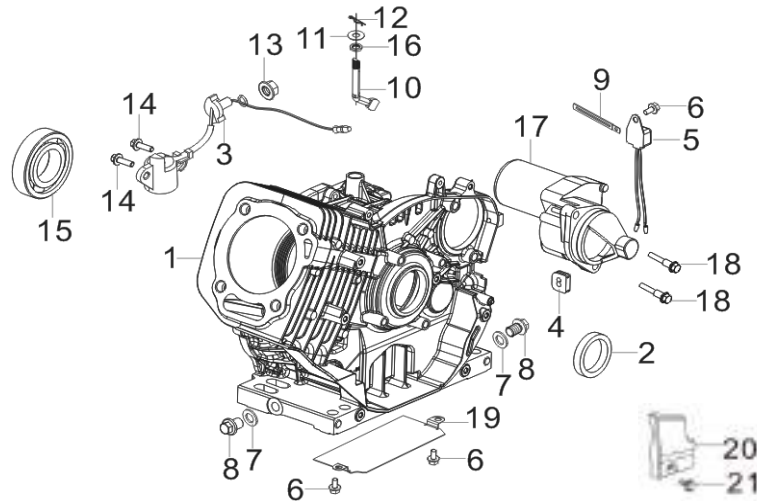
FIG.1 CRANKCASE. / GEAR ASSY, GOVERNOR. (E01)
