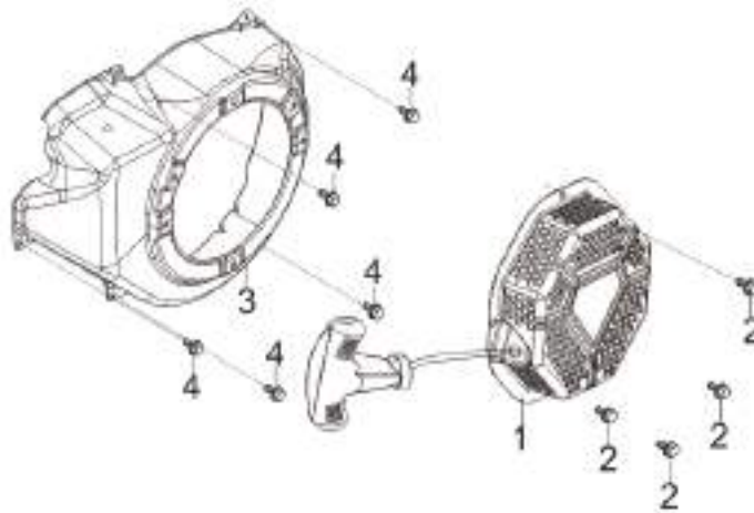
FIG.7 STARTER,RECOIL (E07)
