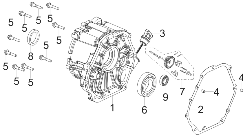
FIG.2 COVER SUBASSEMBLY, CRANKCASE (E02)
