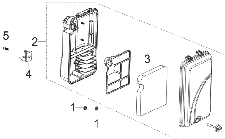
FIG.11 CLEANER, AIR (F01)
