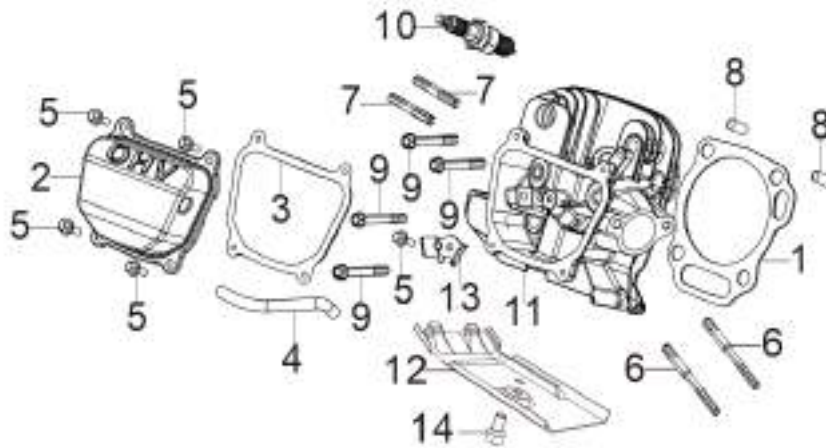
FIG.3 HEAD SUBASSEMBLY, CYLINDER / PLUG, SPARK (E03)
